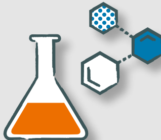
science
