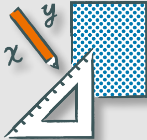
mathematics
